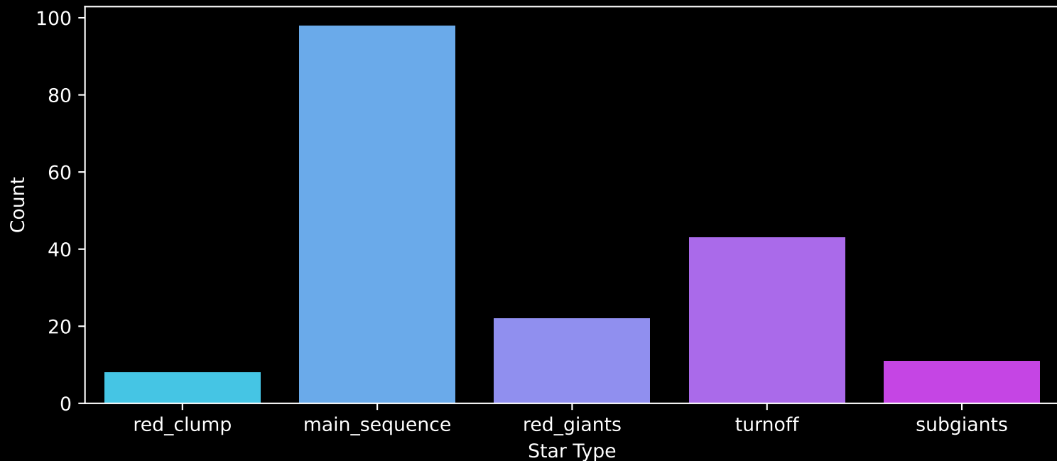
APOGEE DR17 Field: [230+40_MGA] Count plot of Star Type
