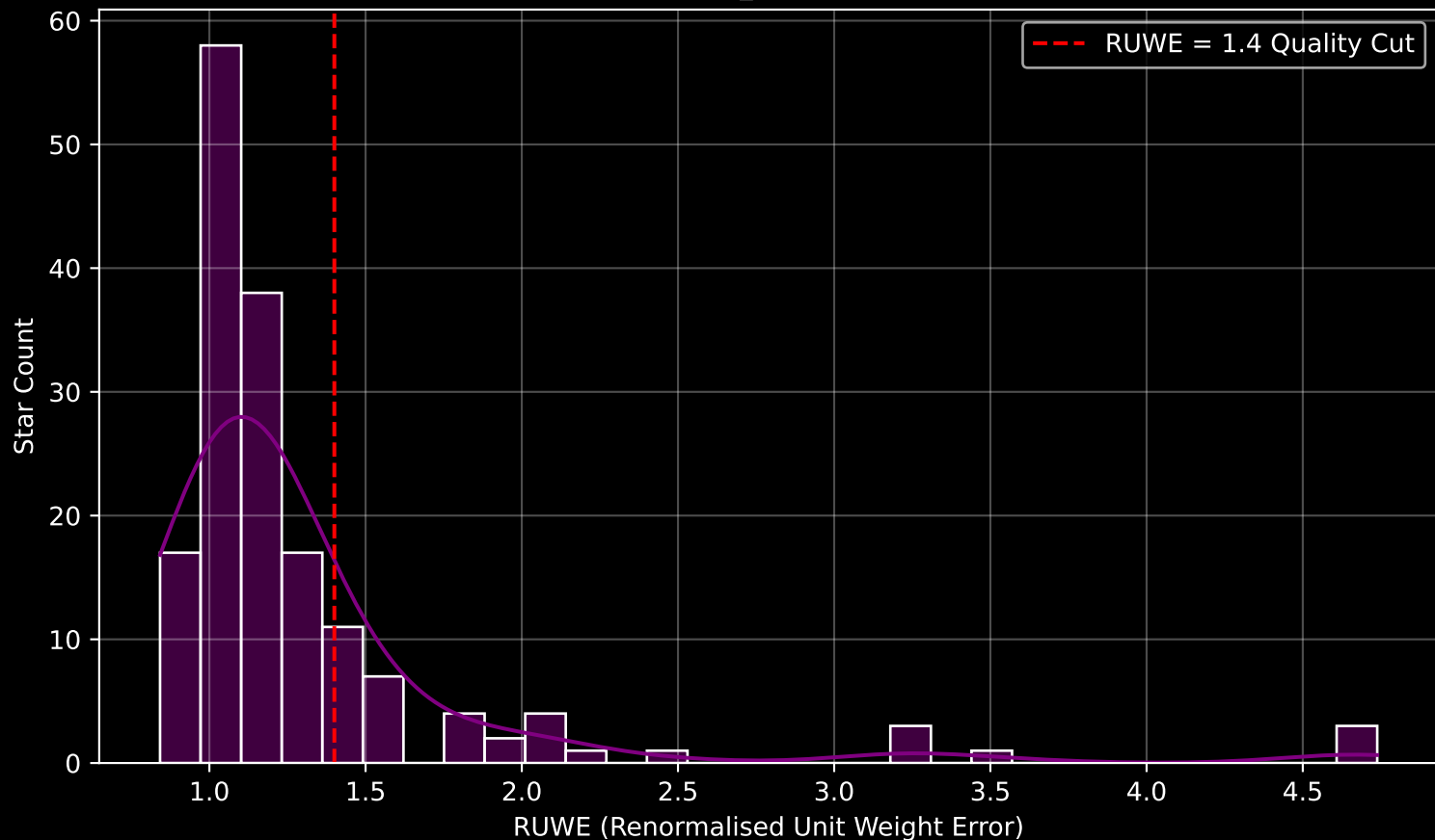
GAPOGEE DR17 Field [230+40_MGA] RUWE Distribution (n= 167)
