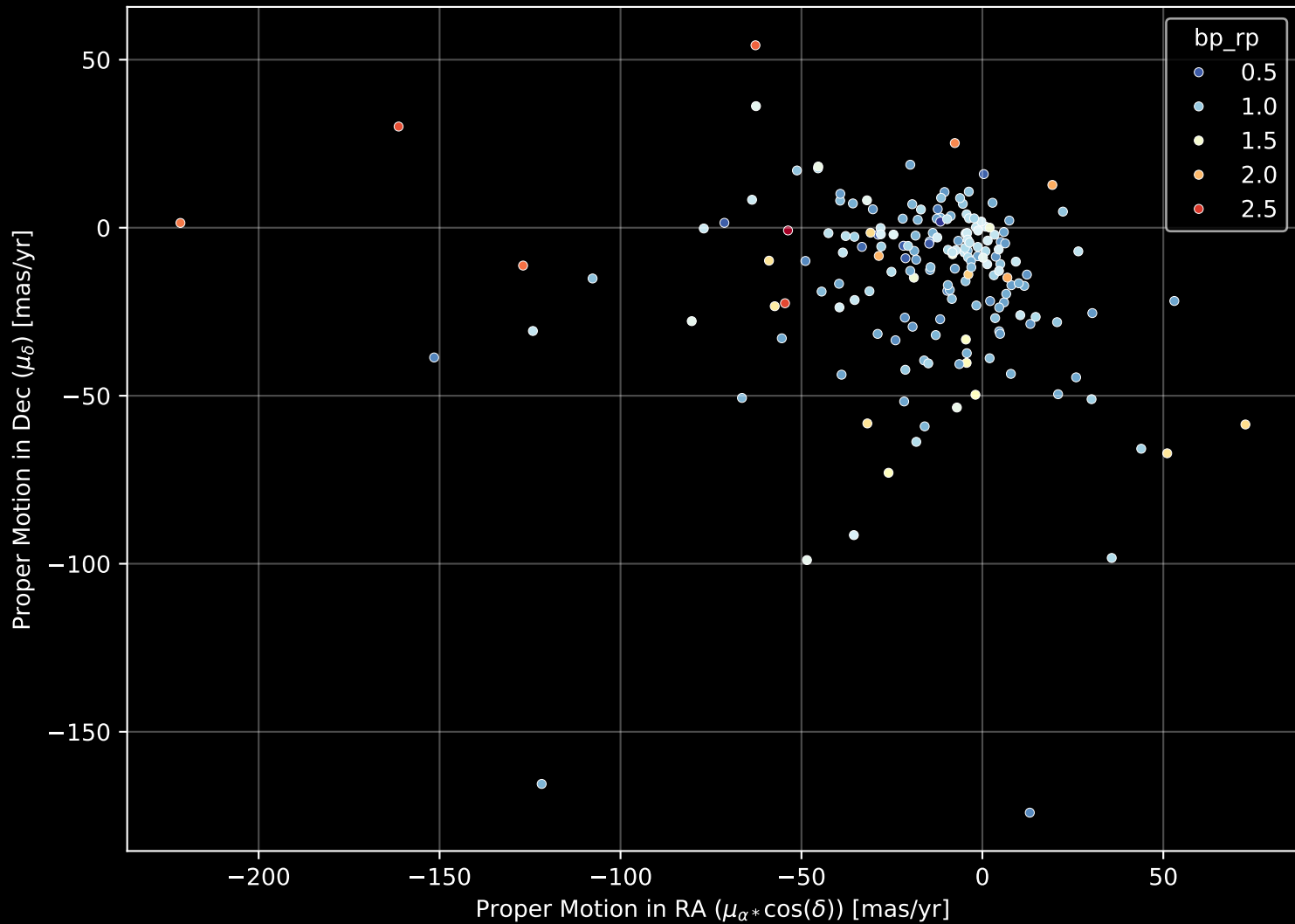
APOGEE DR17 Field: [230+40_MGA] Proper Motion Diagram (n= 182)
