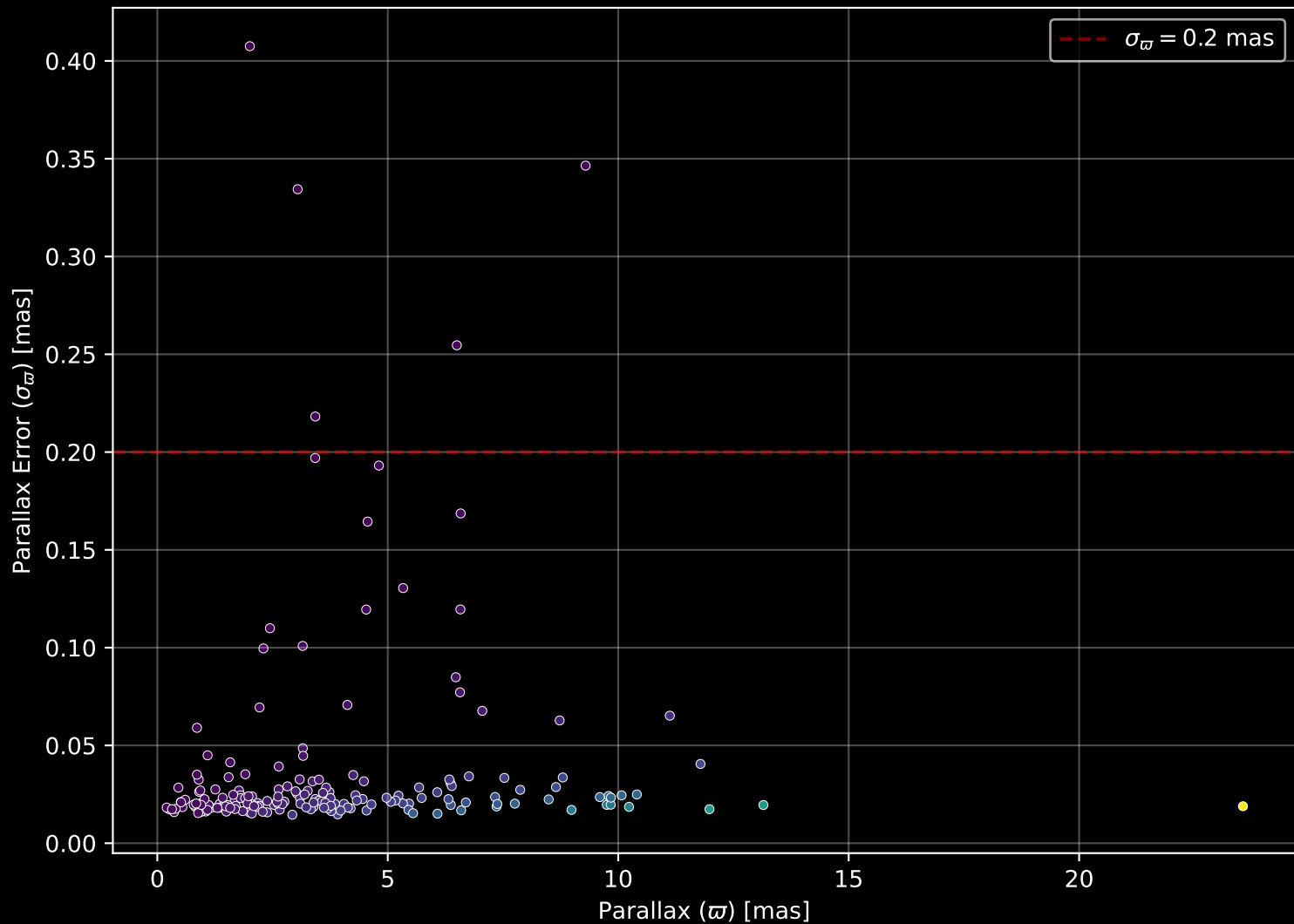
APOGEE DR17 Field: [230+40_MGA] Parallax Quality (n= 182)
