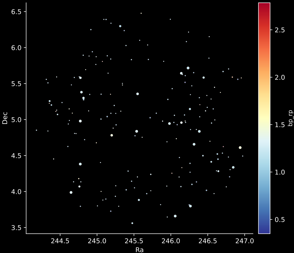
APOGEE DR17 Field: [230+40_MGA] Stars: 182
