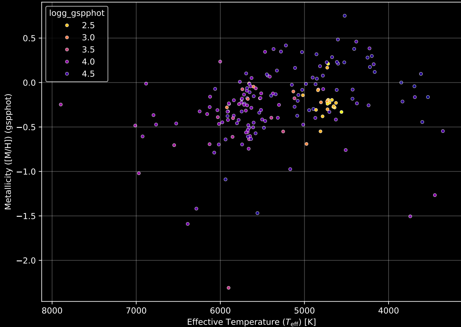
APOGEE DR17 Field: [230+40_MGA] Stellar Population Parameters (n= 182)
